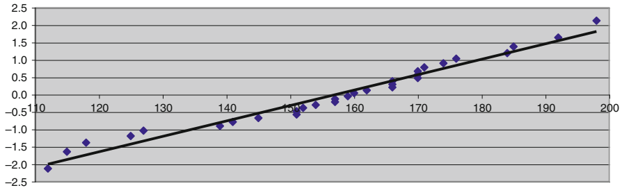
Fig. 4.8 Normal plot
